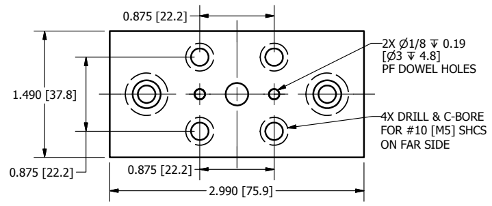
OPTIONAL (-B) END PLATE FOR CONNECTION TO LT-2
