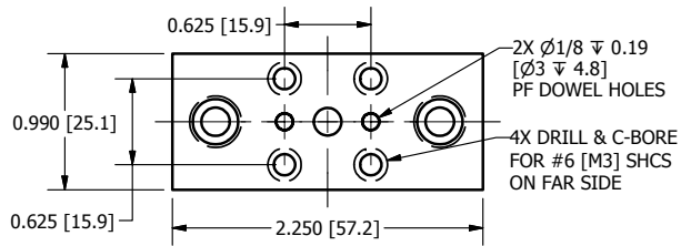
OPTIONAL (-B) END PLATE FOR CONNECTION TO LT-1
